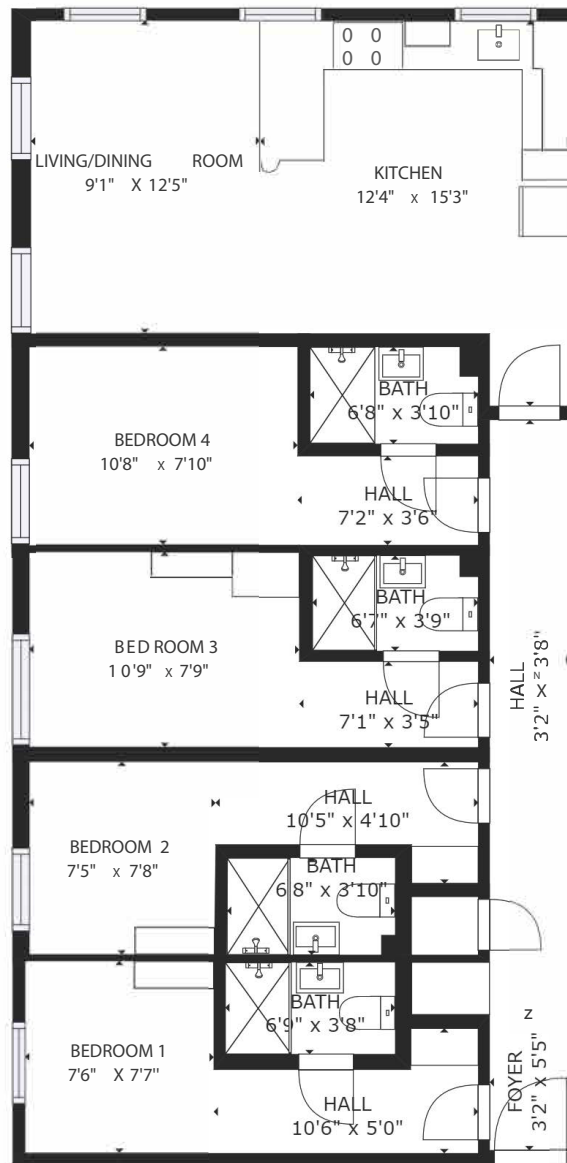
FLOOR 1
